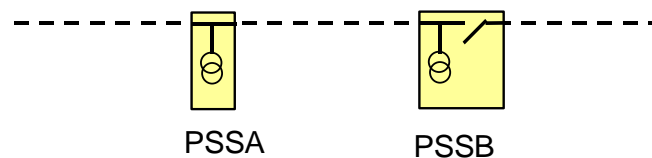
Figure 12 : Schéma non admis (2 tangentes successives sans coupures)
